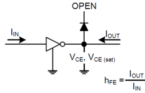
2. V_{CE(sat)}, h_{FE}
